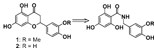
Figure 1. Structural relationship between homoeriodictyol (1), eriodictyol (2), and hydroxylated benzamides of benzylamines (3).
